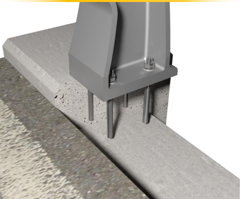
THREADED BAR ANCHORING
