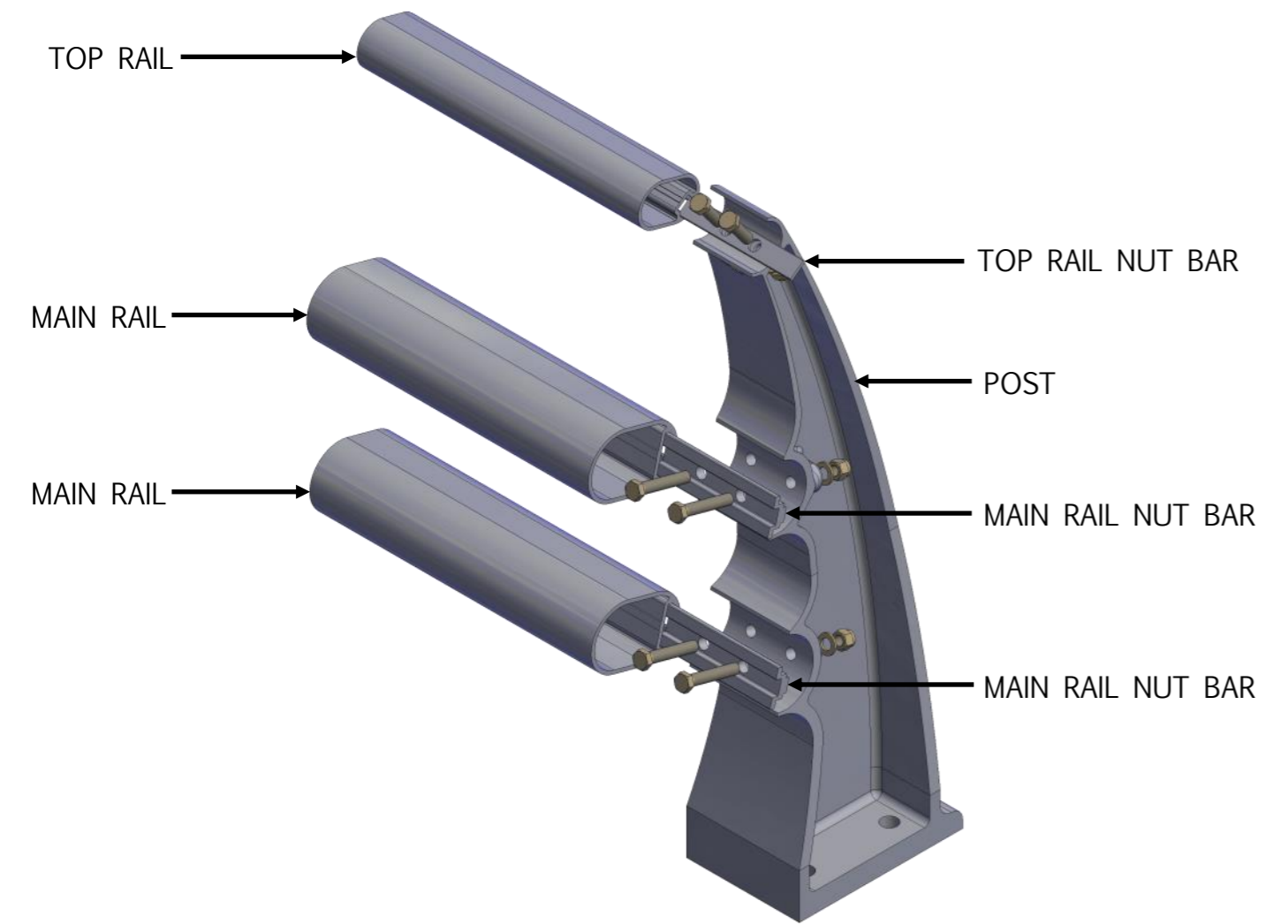
ASSEMBLY VIEW
